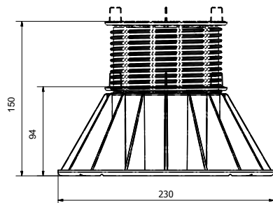
TER09-1183/4F94
